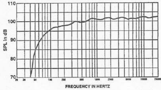
FIGURE 1 — Sx200a Frequency Response (1 watt/1 meter, anechoic environment)
